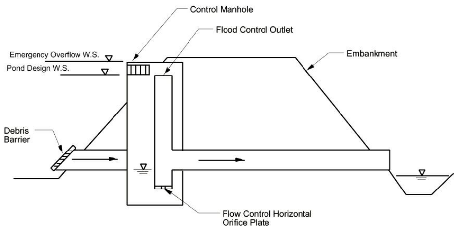
CONTROL MANHOLE WITH SUBMERGED HORIZONTAL ORIFICE PLATE
