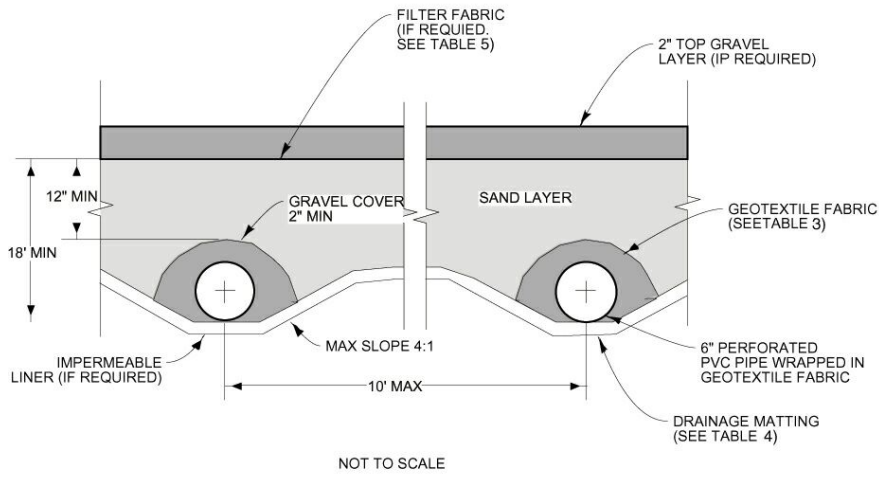
Figure 9B: Filter Bed with Trench Underdrain
