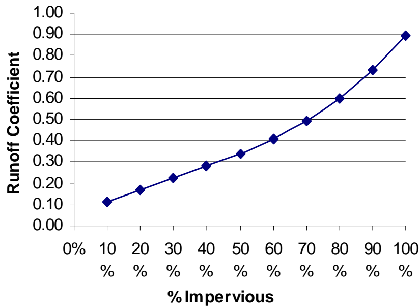
Figure 1. Impervious – Coefficient Curve (WEF/ASCE Method 24 )
