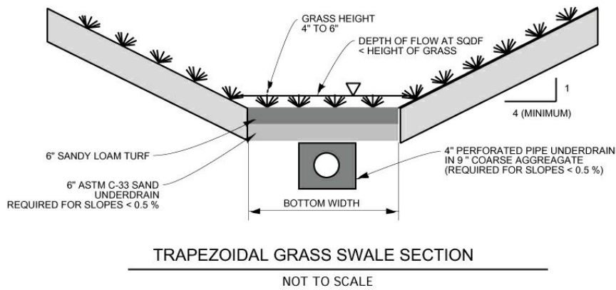
Figure 11: Grassed Swale
